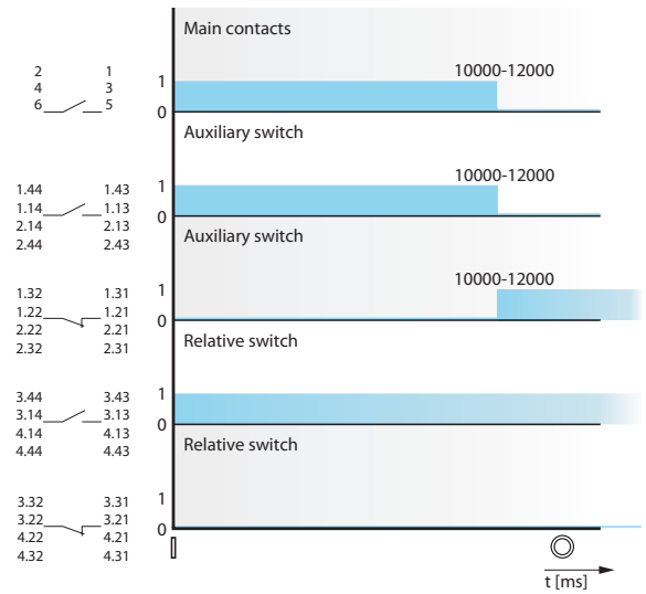
Circuit breaker switched off by motor drive - electrical by push button OFF
