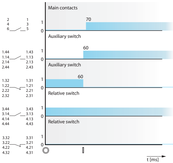
Circuit breaker switched on by motor drive - electrical by push button ON
