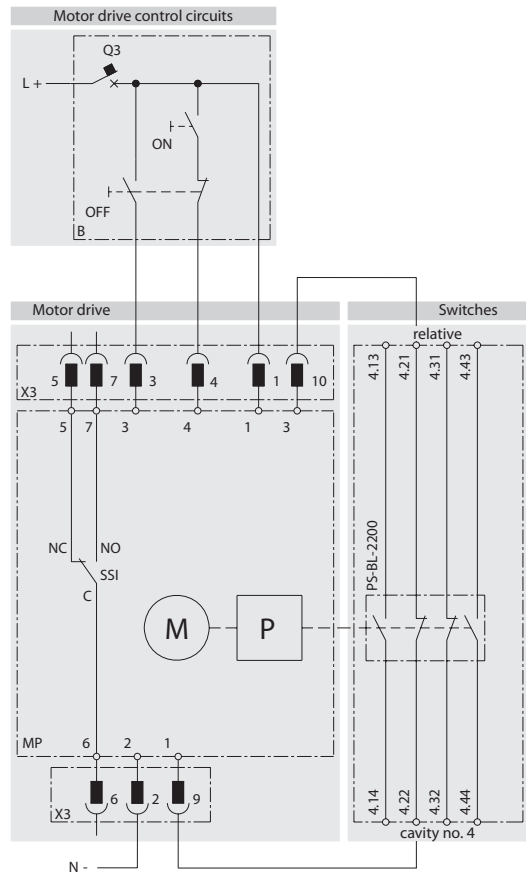
Circuit breaker switch on and switched off by motor driver - electrical by push button ON and push button OFF
